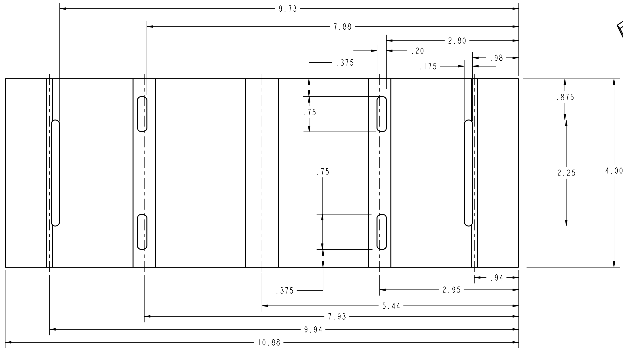
FLAT BLANK PATTERN
